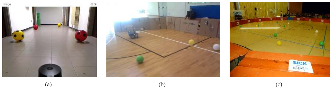
Fig. 7. Environments where Red Beard Button has been tested: the RIMLab Robotics laboratory 1ab (a), the gym of the University of Parma (b), and the Sick Robot Day arena (c).
